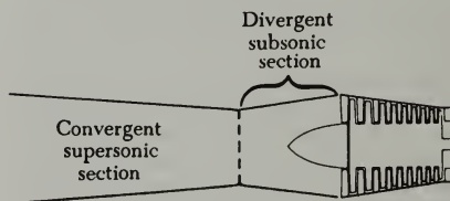
FIGURE 2-22. Supersonic inlet duct.
